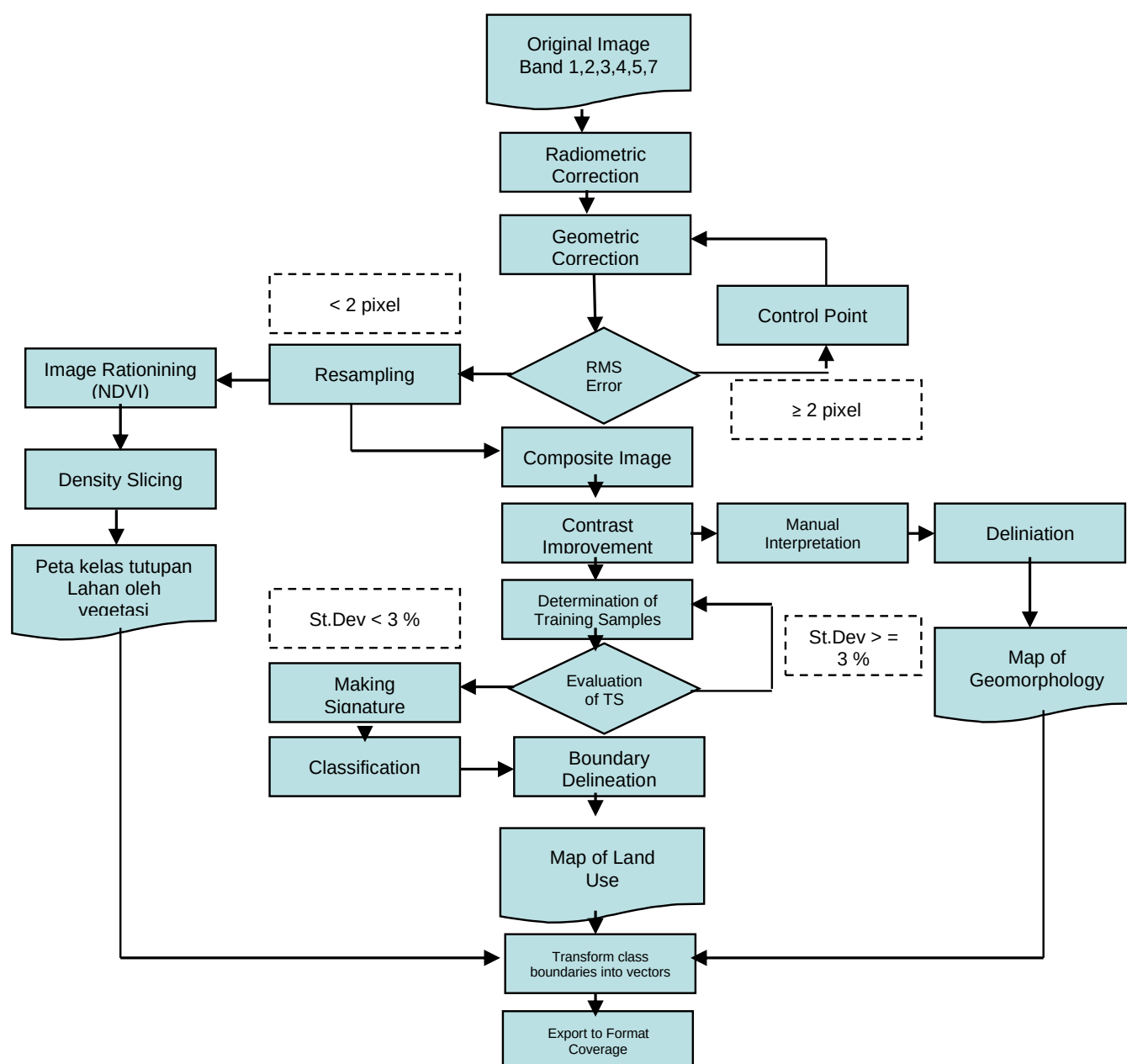
FIGURE 1: Satellite Image Transmission Flow Diagram
