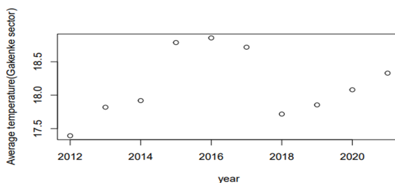
FIGURE 3: Trend of temperature for Gakenke wetland between 2012 and 2021 (Source: RMA, 2024).
