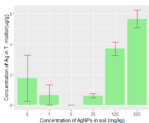
FIG. 5: UPTAKE OF Ag FROM Ag NPs IN SOIL BY A. MOLITOR (n=2).
