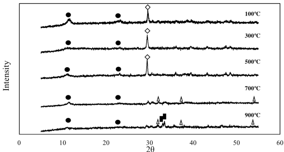
FIGURE 9. XRD Pattern of the Products after Desalination Tests ●: LDH, ◇: CaCO 3 , △: CaO, ■: CaFe 2 O 4
