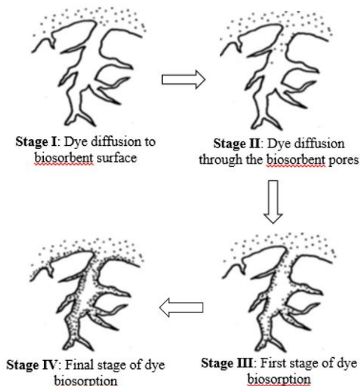
FIGURE 9. PROPOSED FOUR-STAGE MECHANISM OF THE DYE ADSORPTION (SIVAKUMAR 2010)
