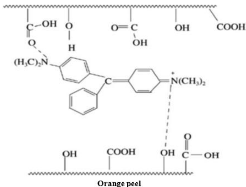
FIGURE 10. PROPOSED MECHANISM FOR THE BIOSORPTION OF THE C.I. BASIC GREEN 4
